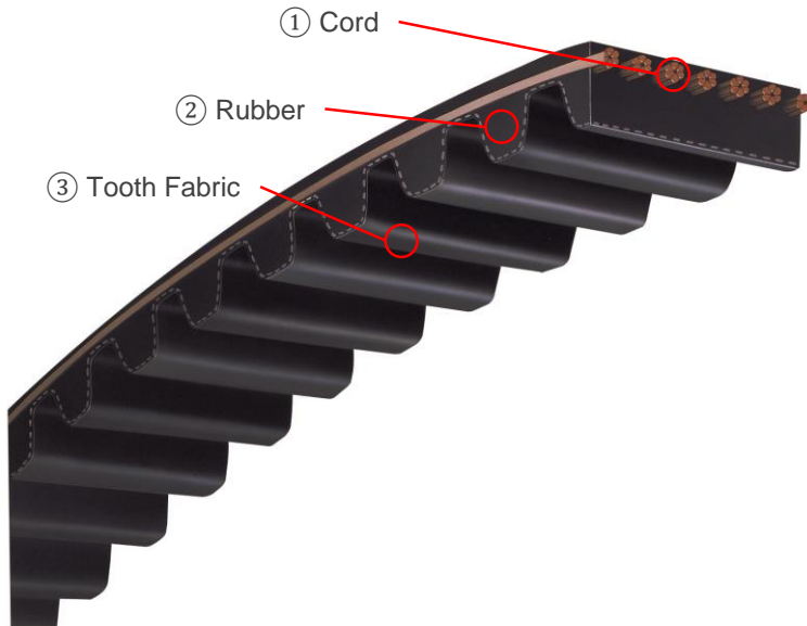
GP8M & GP14M Tooth Profile
