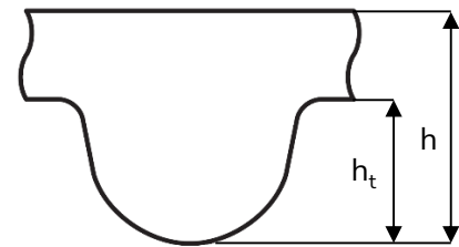
GP8M & GP14M Tooth Profile
