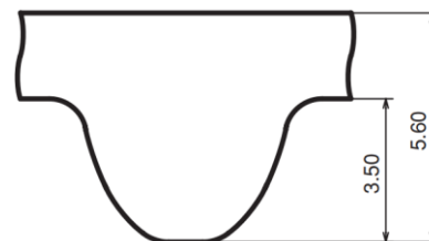
Belt tooth pitch 8mm
