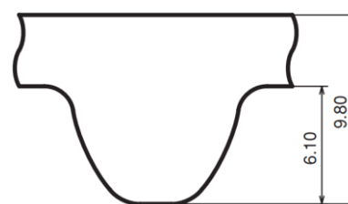
Belt tooth pitch 14mm
